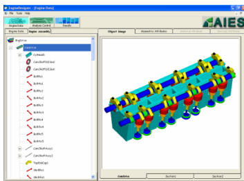
CamDrive object for a V8 gasoline DOHC system
