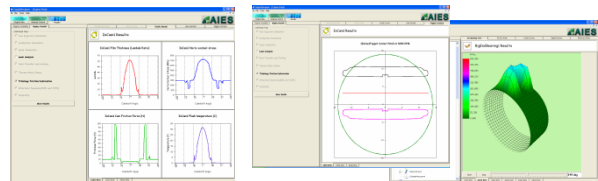
Cam & tappet (CTL) and cam bearing tribology results
